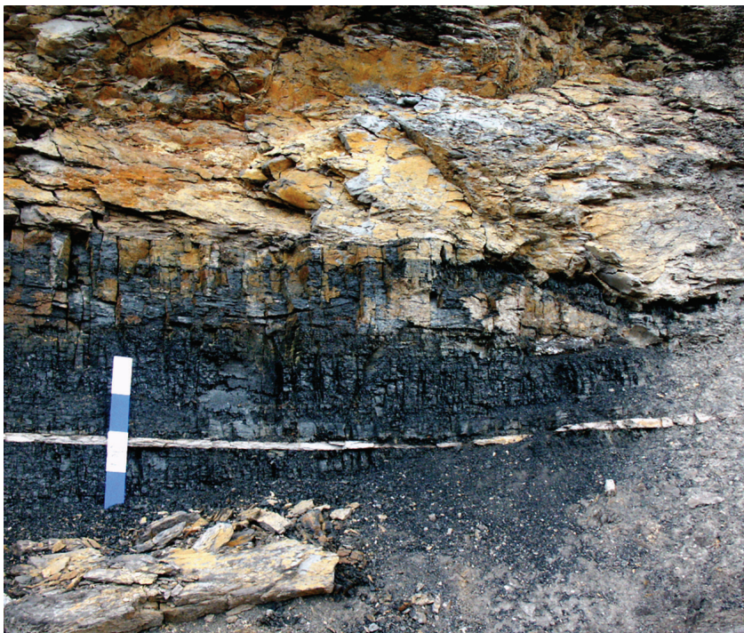
Coal beds near Price, Utah
